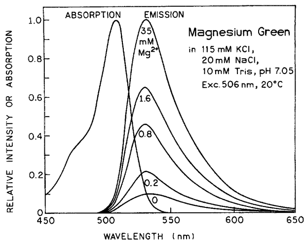
Fig. 3. Absorption and emission spectra of magnesium green.
