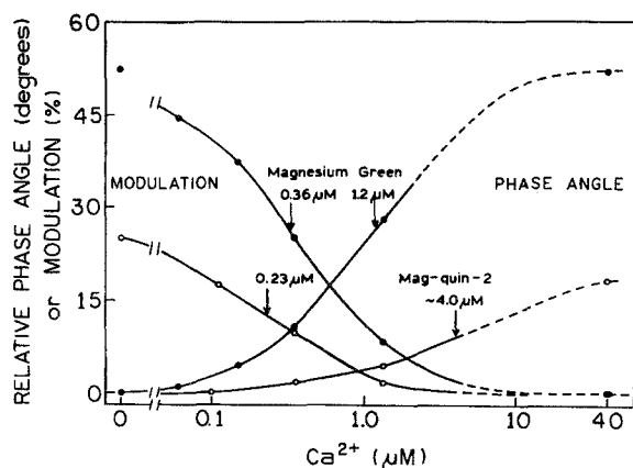
Fig. 10. Ca^{2+} -dependent phase angles and modulations for mag-quin-2 ( \circ ) and for magnesium green ( \bullet ). Arrows indicate apparent dissociation constants (midpoints). Experimental conditions are the same as indicated in the legend to Fig. 7.
